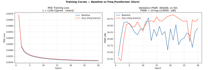
Fig. 2. Training MSE loss (left) and validation PSNR on BSD68 (right) over 30 epochs. Our Freq-Pureformer (orange) converges to a consistently higher PSNR than the spatial-only baseline (blue) while both reach similar training loss levels.
